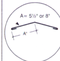
FA-6 FA ridge cap
