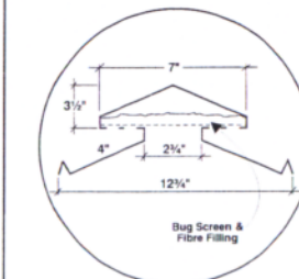
VicWest Vented Ridge
