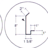
Fascia
